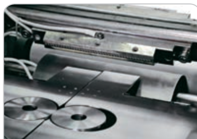
Cross cut sealing system with 2 jaws per shaft
